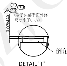
DETAIL "I"
